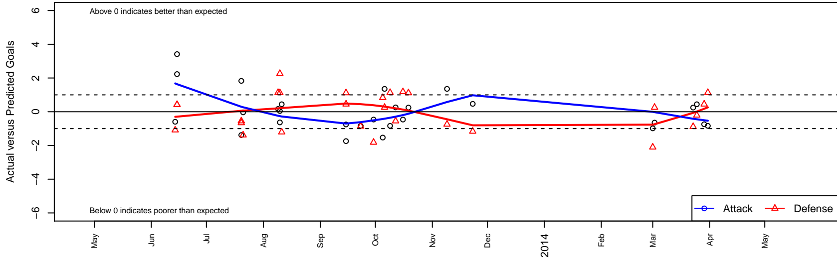
XiFA G2020 G01 Dots are actual minus expected GF (blue circles) and GA (red triangles). Blue line is smoothed change in attack strength. Red is smoothed change in defense strength.
